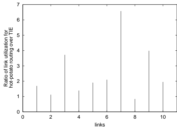
Fig. 8. Comparison of link utilization with hot-potato routing and TIE.
