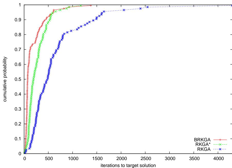
FIGURE 9. Iteration count distributions for BRKGA, RKGA*, and RKGA on instance stn243 with target solution 198.
