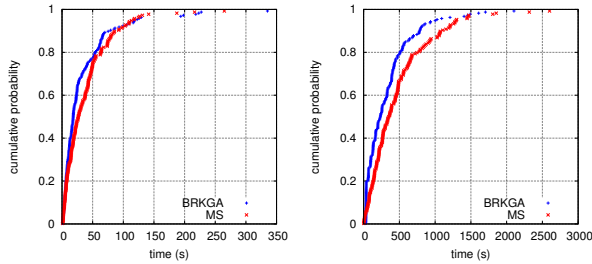
(a) TTT plot for the instance 010_050_025_090. (b) TTT plot for the instance 025_150_225_070.
