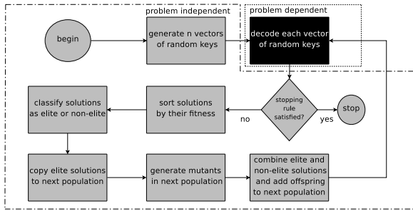
Figure 2: Flowchart of a BRKGA.
