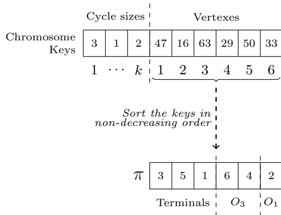
FIGURE 2. Example of solution extraction.
