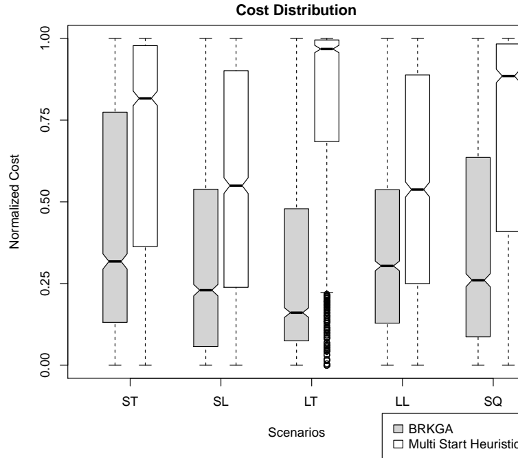
FIGURE 3. Boxplot of the medians and quartiles for each algorithm in each scenario.
